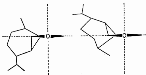
FIGURE 1 Octant projections of norcubebanone (XVIIIa; left) and its C-6 epimer (XVIIIb; right)
